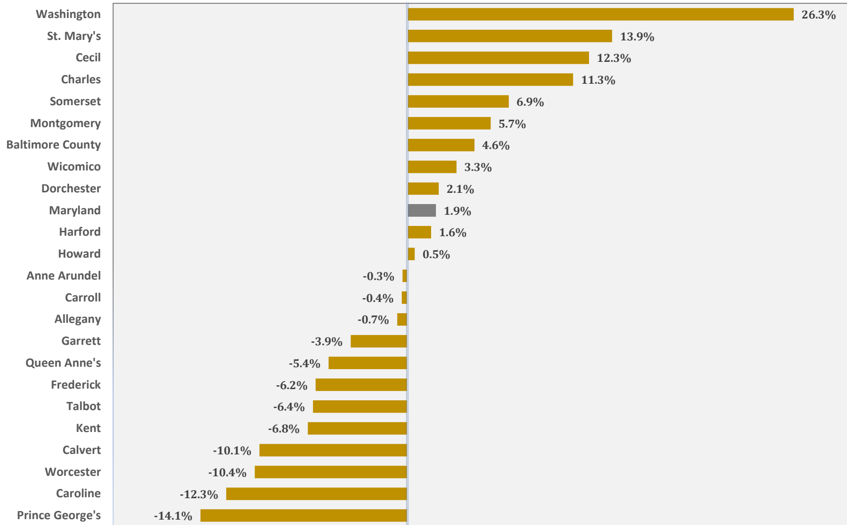
Chart 19: Percent Point Change in Improved Residential Parcels Developed Inside PFAs for Maryland's Jurisdictions, (2013-2021 Share minus 1999-2012 Share )*
